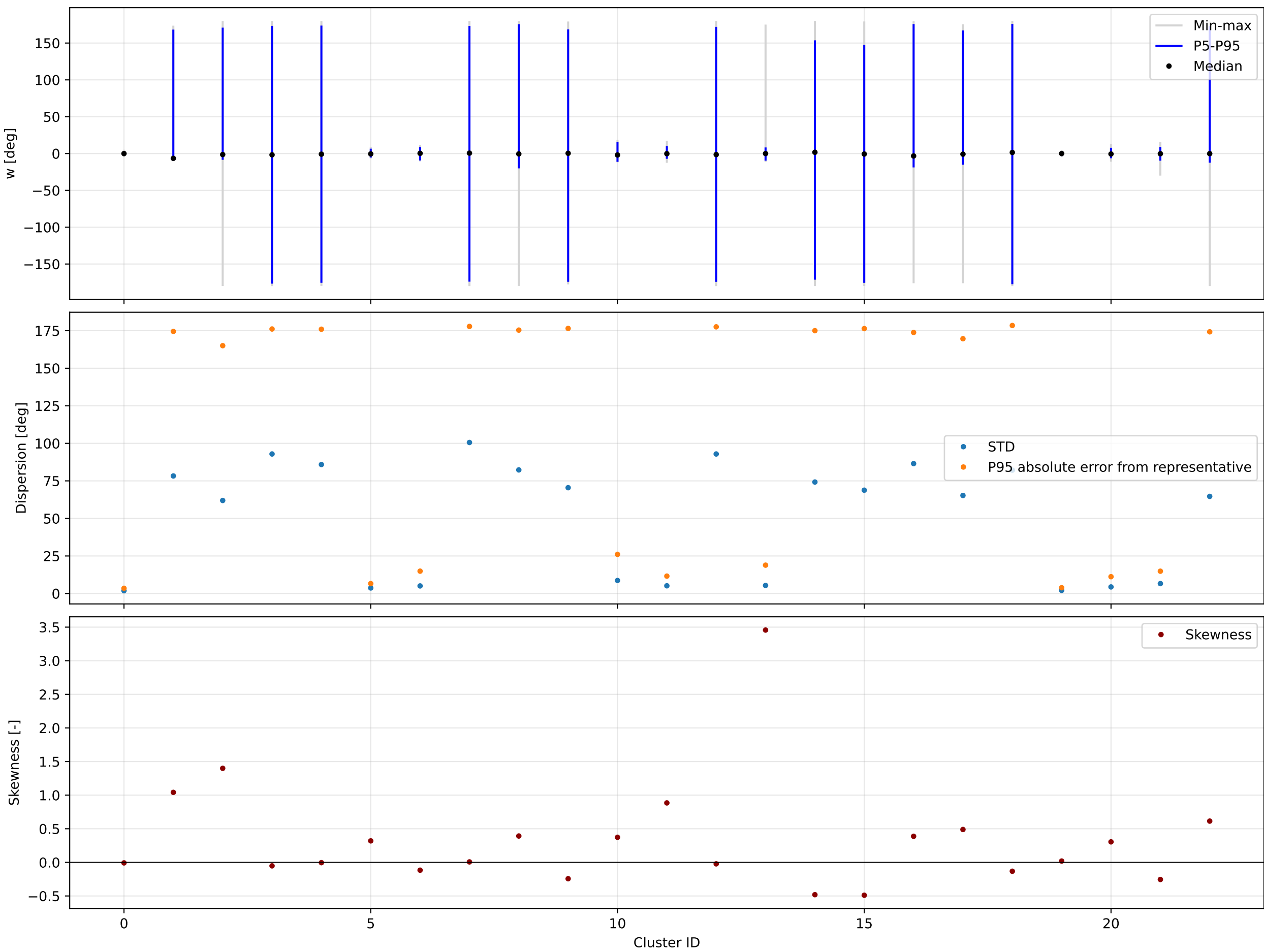
K=23 | backward | w | valid=194058/194058 | offsets from each cluster circular mean
